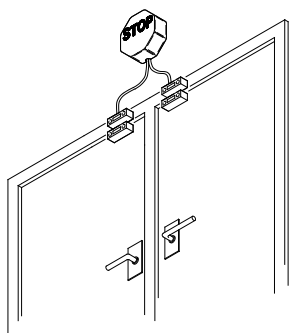
TYPICAL DOUBLE DOOR INSTALLATION STI-6402
