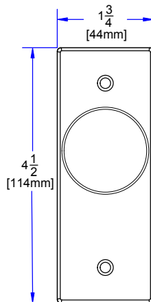
MULLION FACEPLATE
