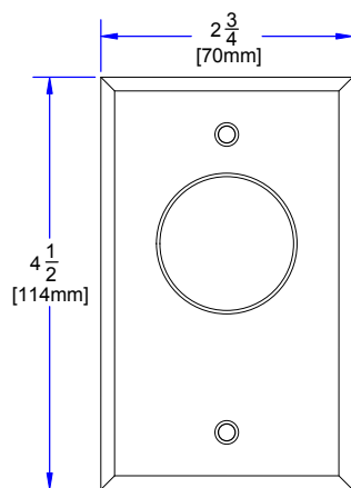
SINGLE GANG FACEPLATE
