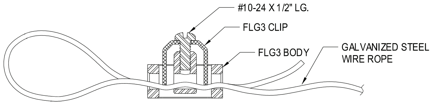
CROSS SECTION ASSEMBLY VIEW
