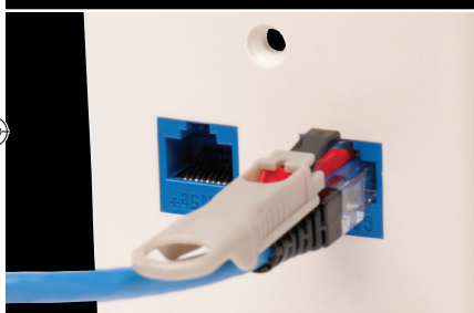
Remove lock with key to unplug connector
