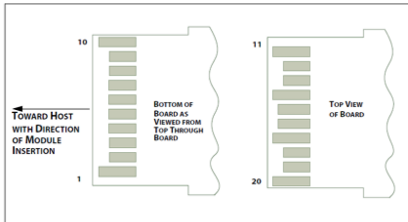
Figure 2. Module Interface to Host
