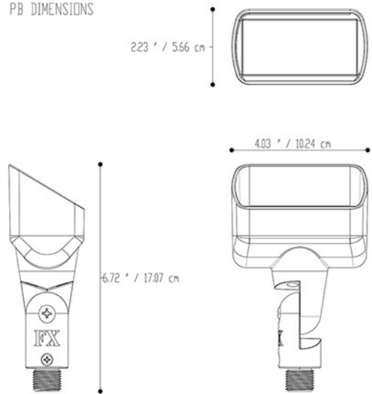
PB DIMENSIONS
