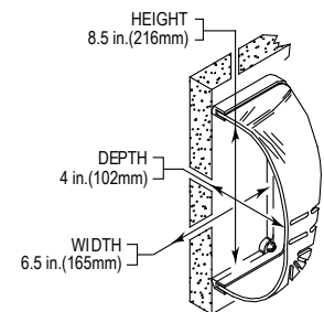
INTERNAL DIMENSIONS
