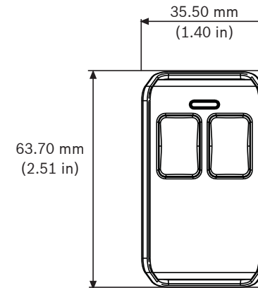
RFPB-TB 2-button
