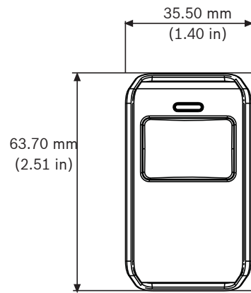
RFPB-SB 1-button
