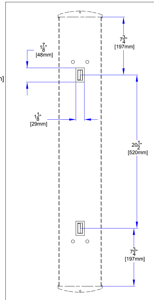
CM-7536 with Kinetic Wall Mounting Back View
