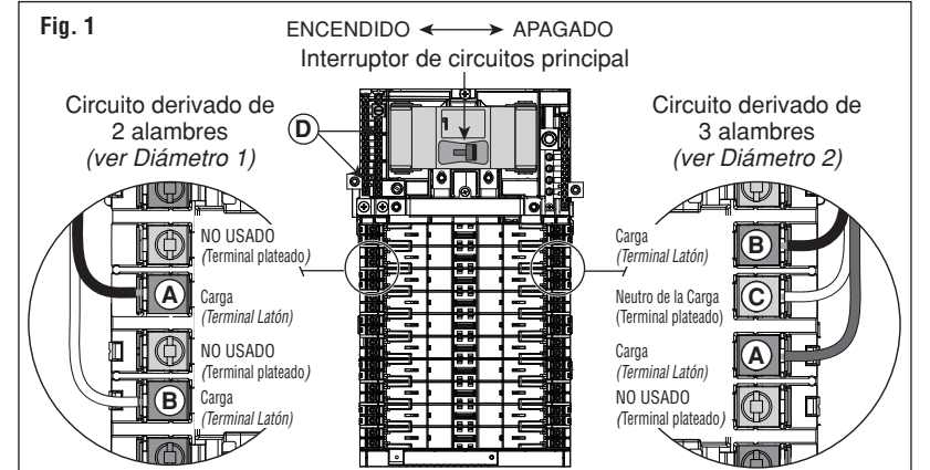
Dia. 1 2 polos, 2 alambres 120/240 VCA
