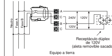
Dia. 2 2 polos, 3 alambres 120/240 VCA
