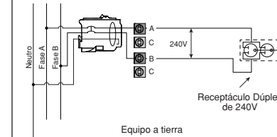
Dia. 1 2 polos, 2 alambres 120/240 VCA
