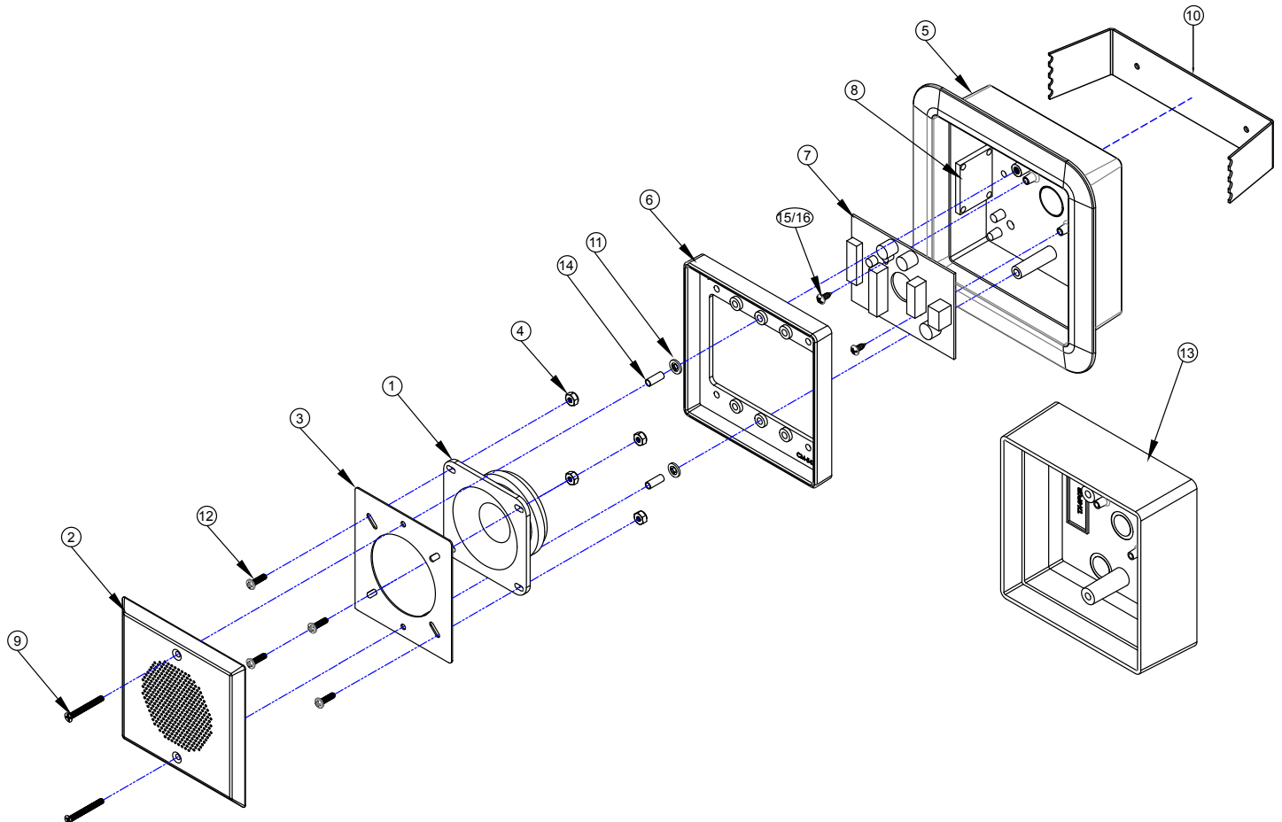
Figure 9.1 - Exploded View
