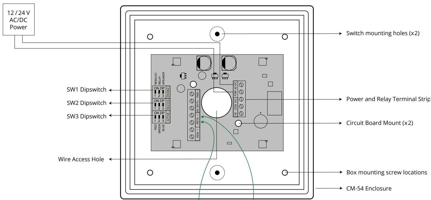
Figure 6.2 - CM-54i Wiring Diagram (Typical)
