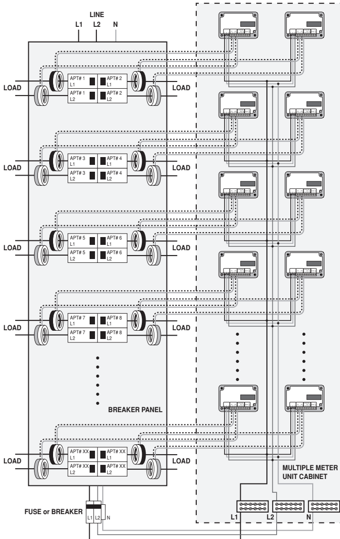
Figure 11: 2-Phase (split phase), 3-Wire Hookup Diagram
