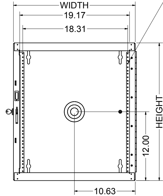
FRONT VIEW (without Door)
