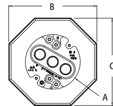
6.8 cu. in. 8131, 8141, 8151, 8161, 8171
