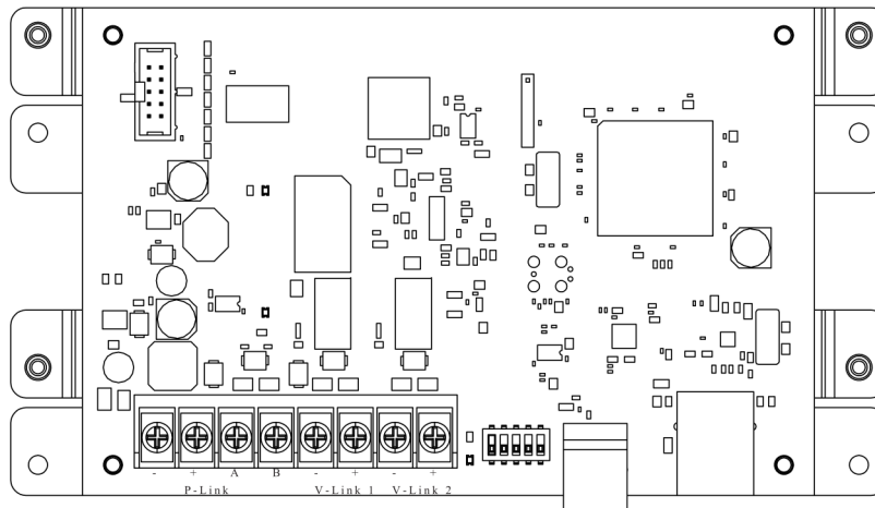
Figure 5. RM-1000ECS Connections
