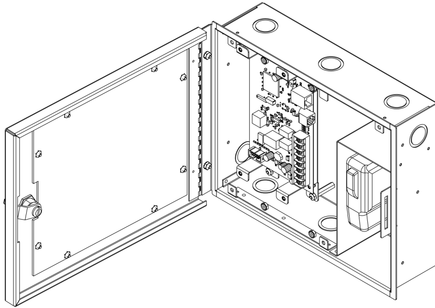
Figure 4. RM-1000ECS Installation
