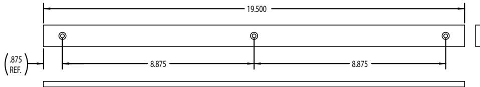
Model LCR-20RK
