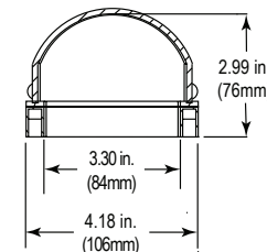
END VIEW STI-6520 STI-6521 STI-6522
