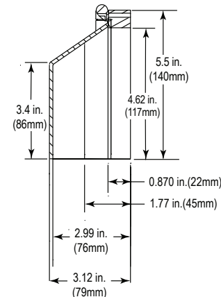
SIDE VIEW STI-6522
