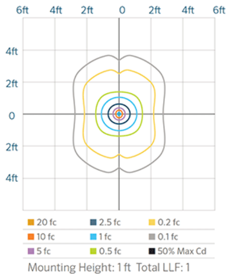
TM LED 20W ISOFOOTCANDLE PLOT
