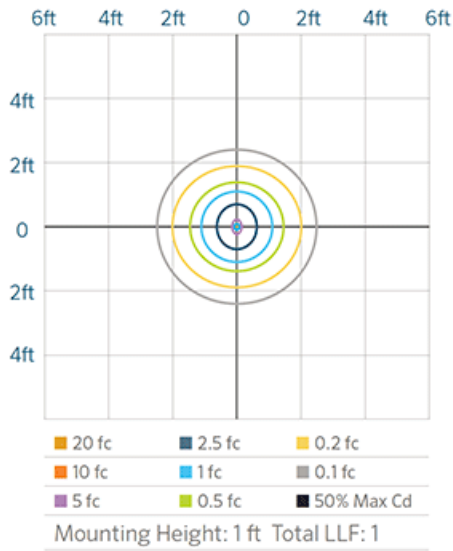
DM LED 10W ISOFOOTCANDLE PLOT
