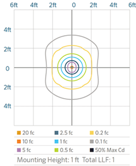
PL LED 20W ISOFOOTCANDLE PLOT
