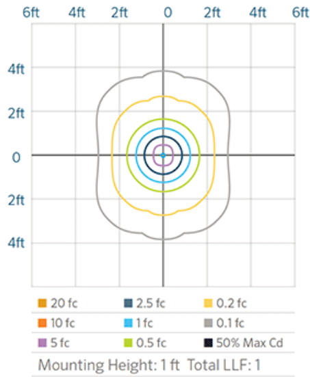
DM LED 20W ISOFOOTCANDLE PLOT
