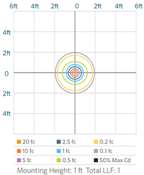
TM LED 10W ISOFOOTCANDLE PLOT
