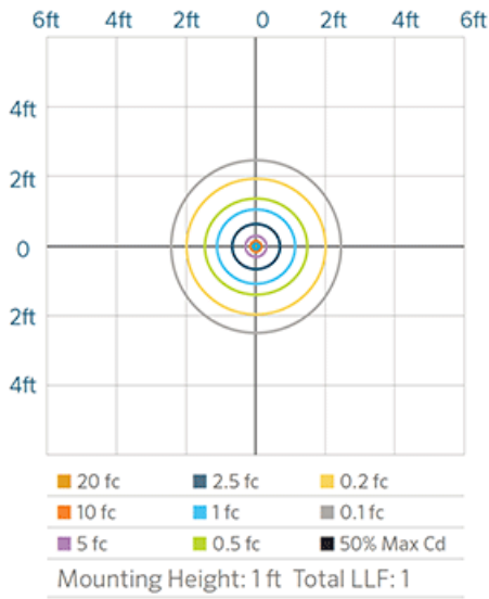
DL LED 10W ISOFOOTCANDLE PLOT
