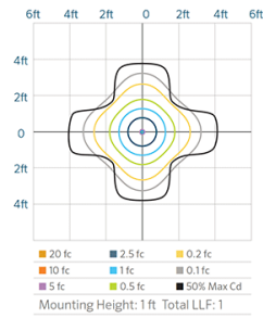
SP LED 20W ISOFOOTCANDLE PLOT
