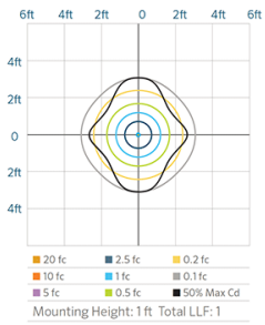
SP LED 10W ISOFOOTCANDLE PLOT
