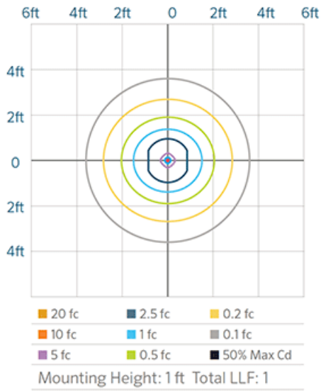
PL LED 10W ISOFOOTCANDLE PLOT
