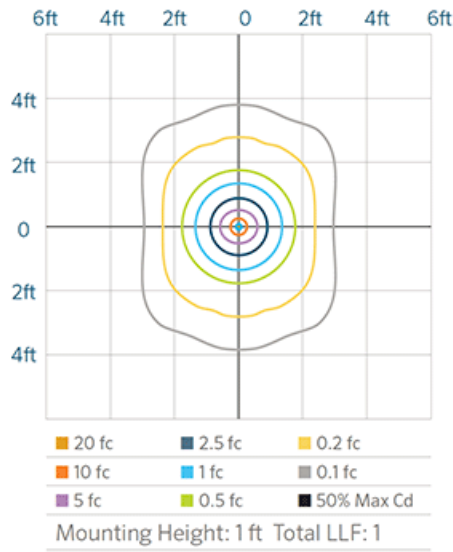
DL LED 20W ISOFOOTCANDLE PLOT
