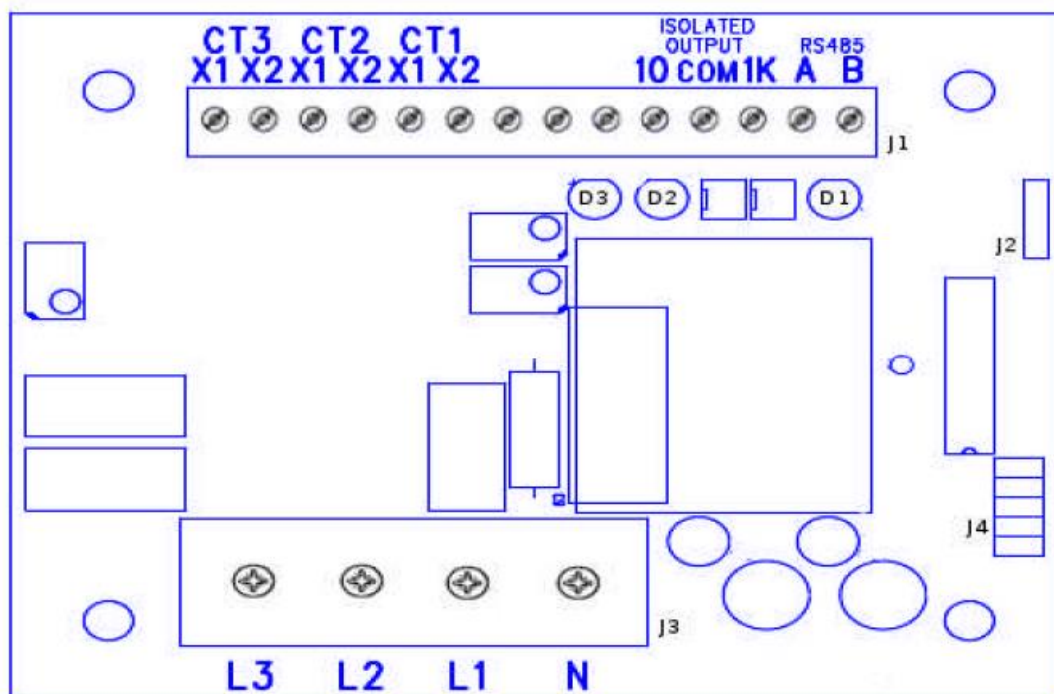
Figure 1: Series 2000 terminals
