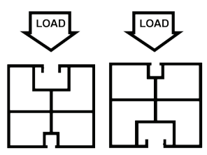
Load resistance between large channel and small channel is substantially the same.
