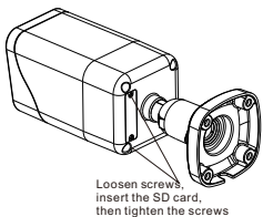
Figure 3-3 Installing SD card
