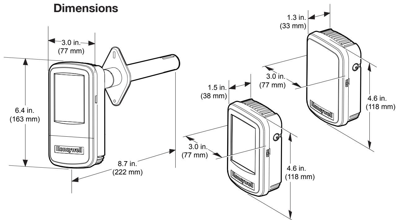
Figure 8. Monitors' dimensions
