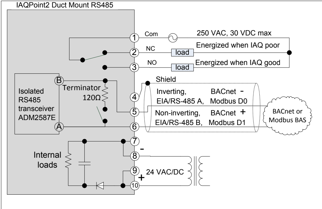
Figure 11. Wiring schematics for RS-485 duct-mount units
