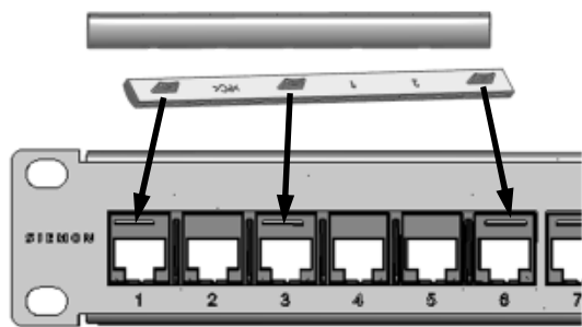
Icon/label holder (6-port wide with keyed slots) p/n: Z-PNL-PS
