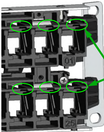
48-port, 2U version
