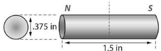
M-16 3/8" Dia. x 1 1/2"
