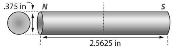
M-3938 3/8" Dia. x 2 9/16"
