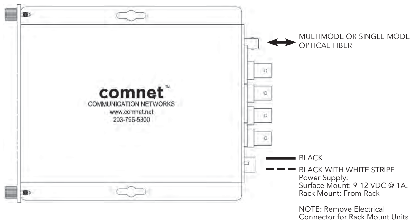
FIGURE 1 - FVT/FVR4012 TRANSMITTER AND RECEIVER
