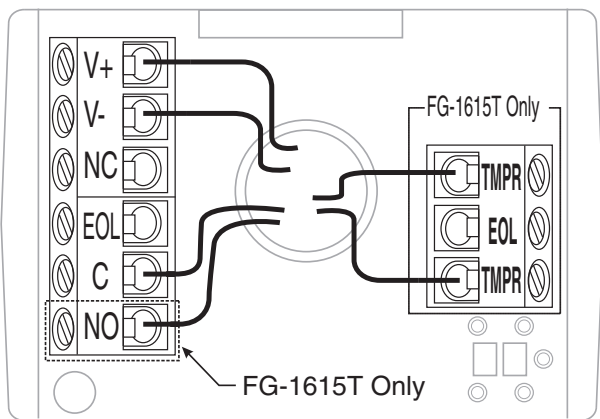
Normally Open Loop/No EOL Resistor
