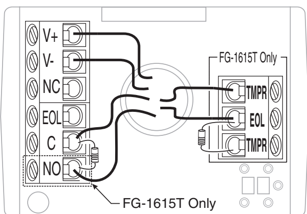
Normally Open Loop/With EOL Resistor
