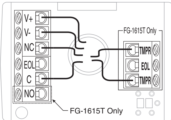
Normally Closed Loop/No EOL Resistor
