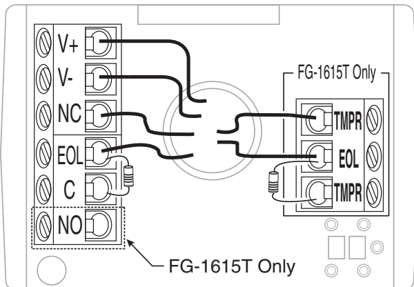
Normally Closed Loop/With EOL Resistor
