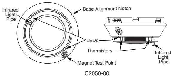
FIGURE 4. CLEANING THE PTIR DETECTOR
