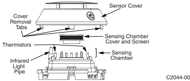
FIGURE 4. CLEANING THE PTIR DETECTOR
