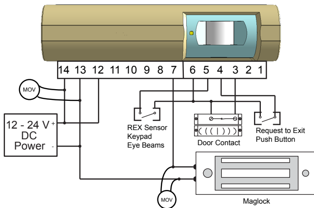
MODE 4 WIRING DIAGRAM
