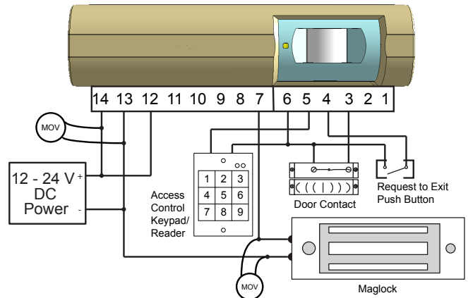
MODE 3 WIRING DIAGRAM
