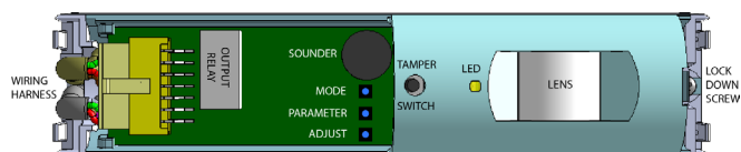
FIGURE 1 - COMPONENT LOCATIONS
