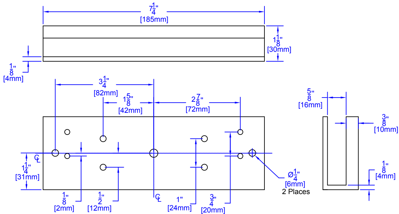
CX-MA0611 Bracket
