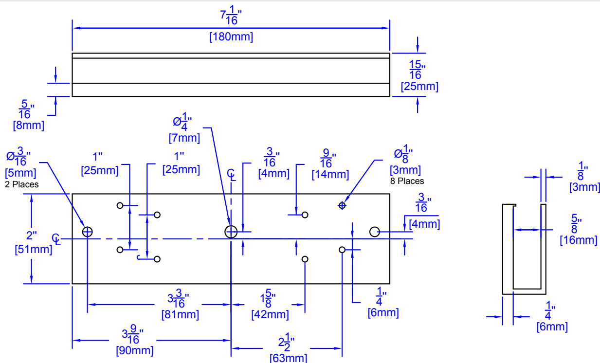
CX-MA0611 Bracket
