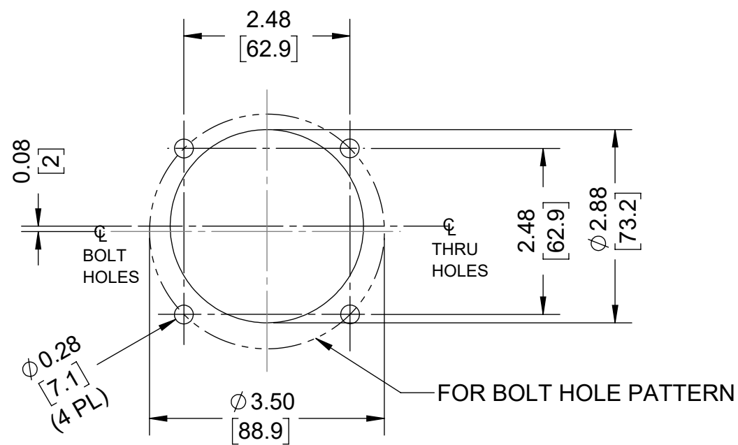
MOUNTING PATTERN FOR 30° MALE & FEMALE PANEL MOUNT RECEPTACLES
