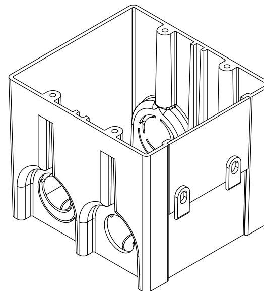
ISOMETRIC VIEW
