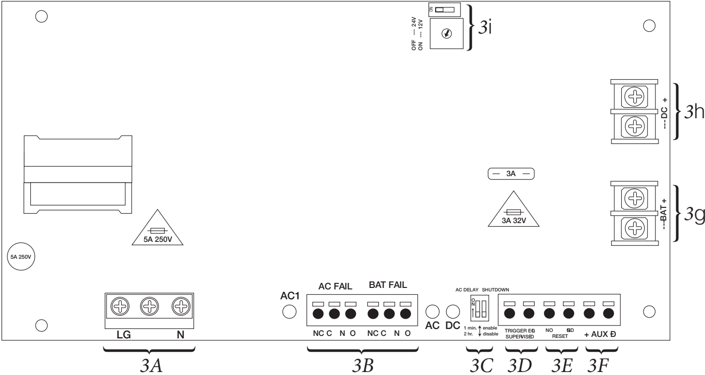
Fig. 3 - eFlowNB Configuration
