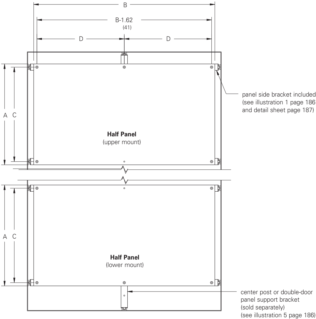
Half Panel Mounting
