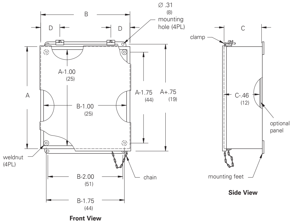
Cover Clamp Layout
