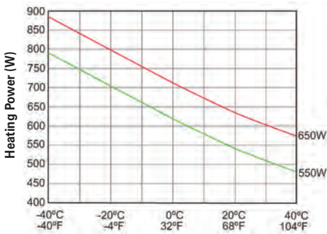
Heating Power / Ambient Temperature at 60Hz
