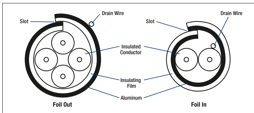
Figure 1: Foil shield configurations without shorting folds.
