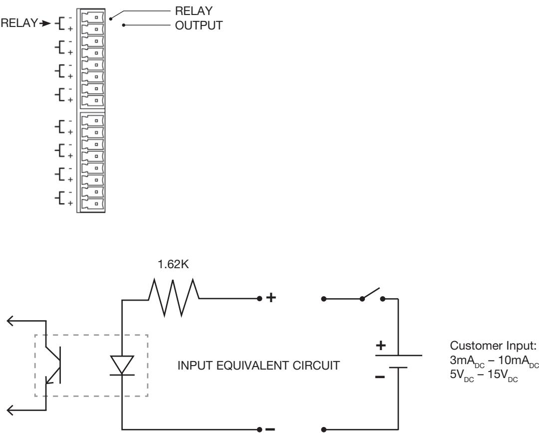
FIGURE 3 – TYPICAL RELAY SETTINGS
