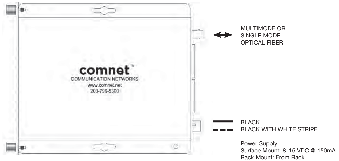
FIGURE 1 – FDC8ISOT TRANSMITTER
