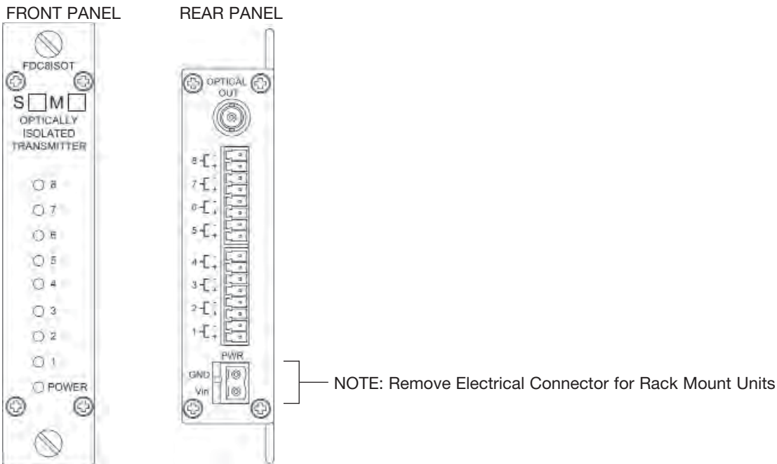
FIGURE 2 – FDC8ISOT TRANSMITTER
