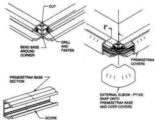
FIG. 10 External Elbow, PT1EE...
