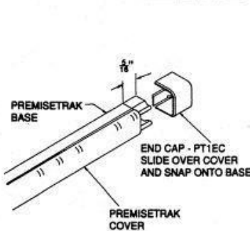
FIG. 5 End Cap, PT1EC...
