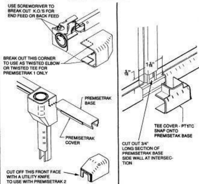
FIG. 12 Tee Cover, PT1TC...
