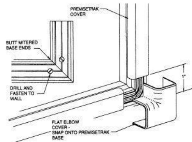
FIG. 7 FLAT ELBOW PT1FE...
