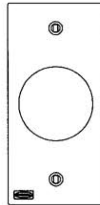
KP720/KP720AL/, KP720GY RECEPT. 1.60 ID
