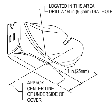
WEEP HOLE INSTALLATION
