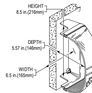
INTERNAL DIMENSIONS
