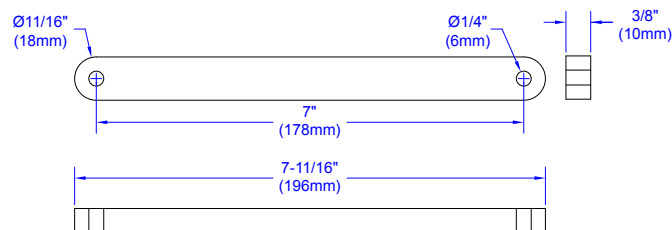
7" Extension Bar
