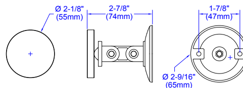
Armature Plate
