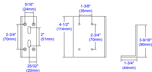
Floor Mount L Bracket
