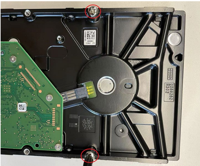
Figure 4 Lock Screws for HDD(s)
