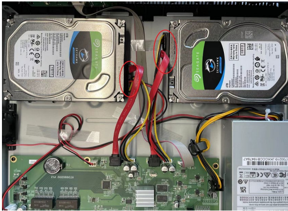
Figure 6 Connect HDD(s)
