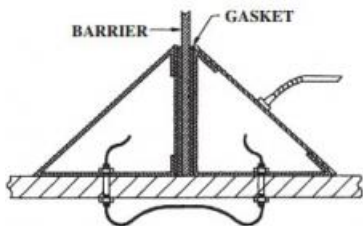
"B" TYPE MOUNTING
