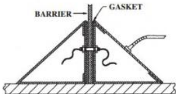
"B" TYPE MOUNTING
