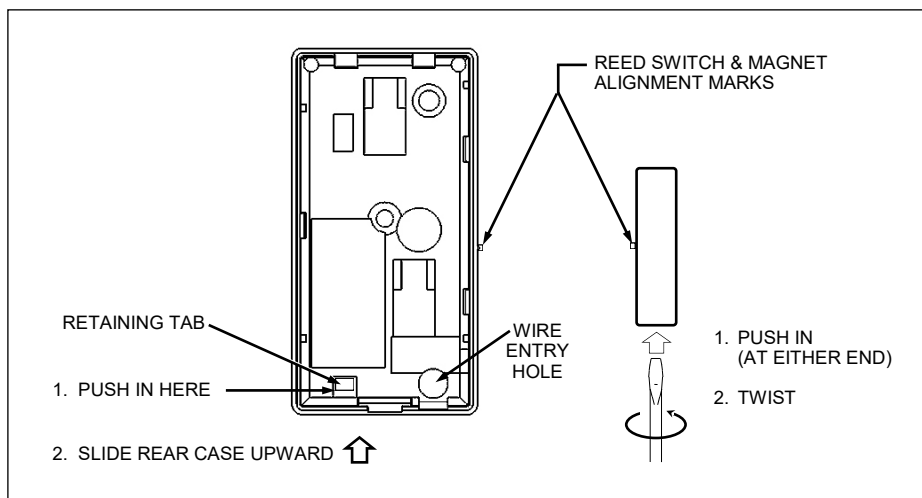
Fig. 5. Removing Mounting Plate and Magnet Cover
