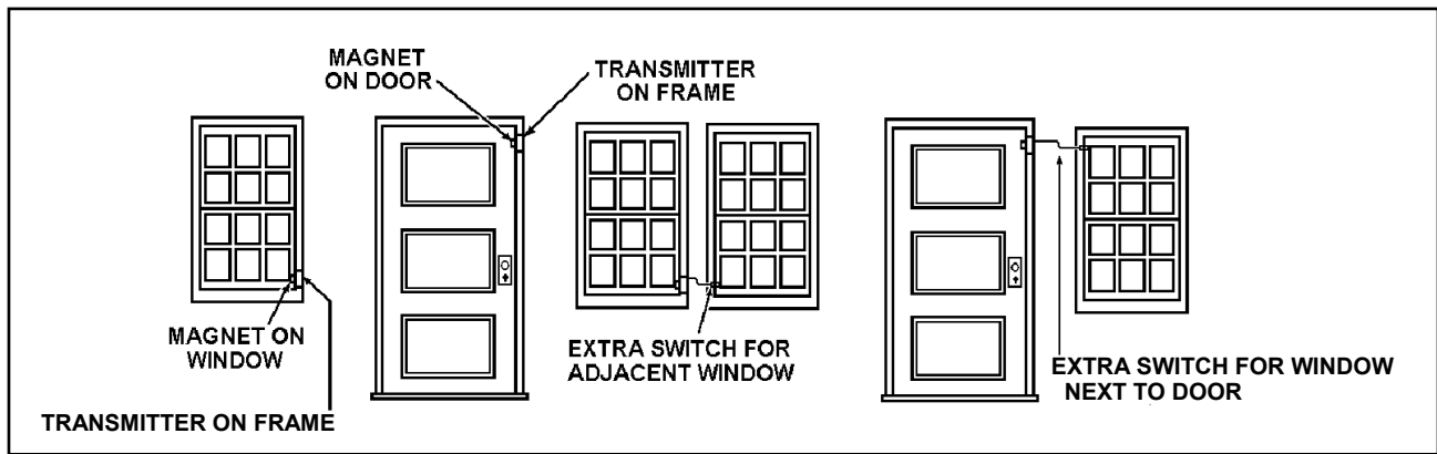
Fig. 6. Typical Transmitter Locations
