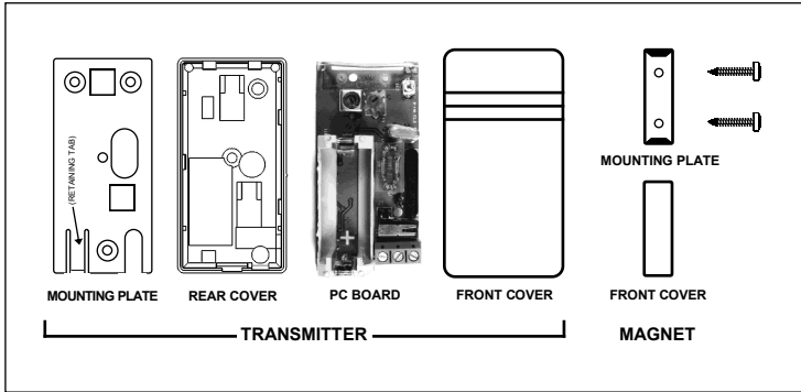
Fig. 1. Component Parts
