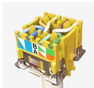
Step 3 Cables laced and trimmed
