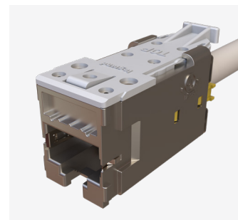
Step 4 Full jack body with lacing cap inserted
