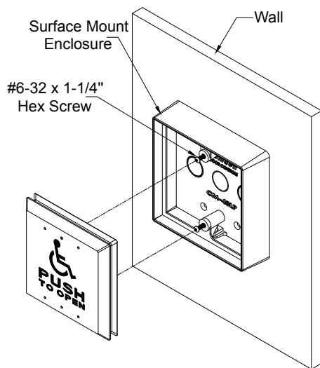
CM-45K Surface Mount
