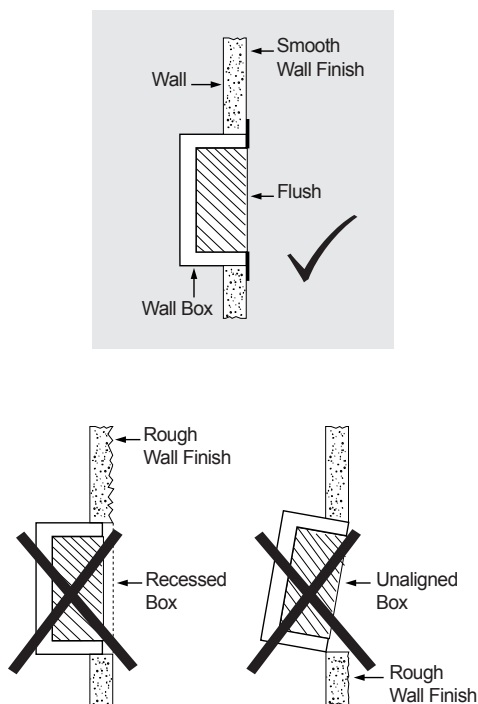
Figure 2.1 - Proper Box Installation
