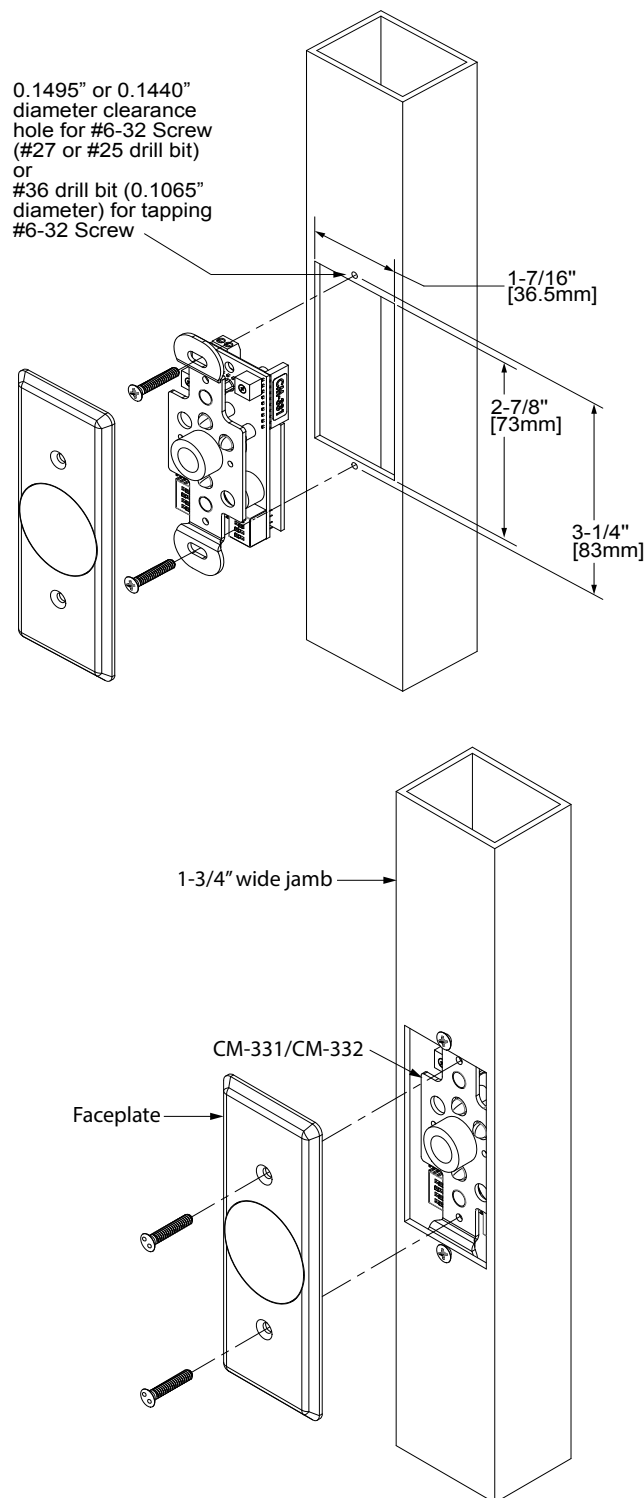
Figure 2.2 - Installation for 1-3/4" Jamb
