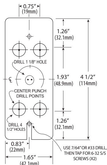
CUTTING TEMPLATE
