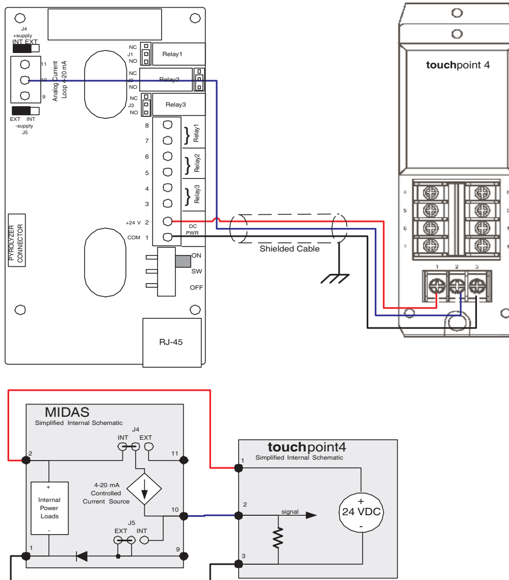
Diagram 4-21. Midas® to Touchpoint4 3-Wire Sourcing Connection
