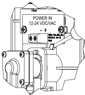
CONTACT REMOVAL DETAIL A
