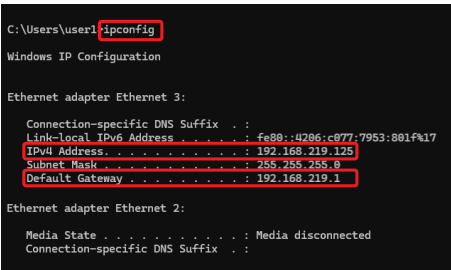
<Command Prompt screen example>
