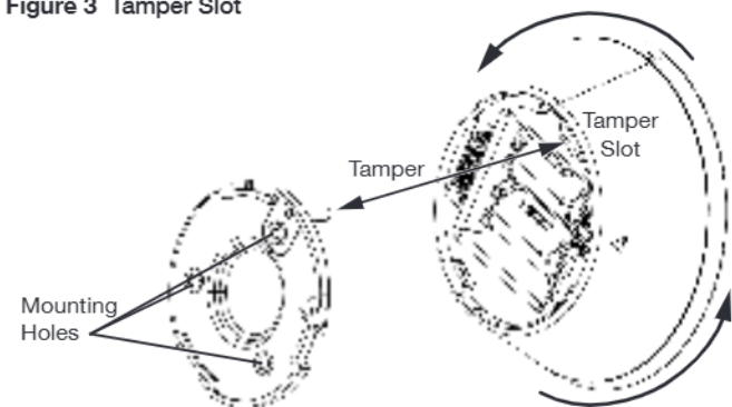
Figure 3 Tamper Slot
